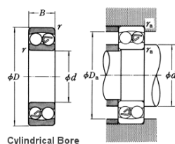
Cylindrical Bore
